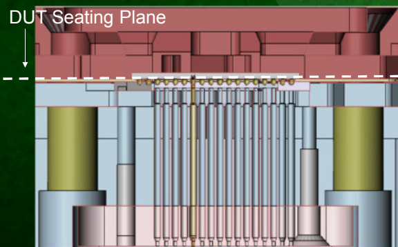
xWave Package Test
