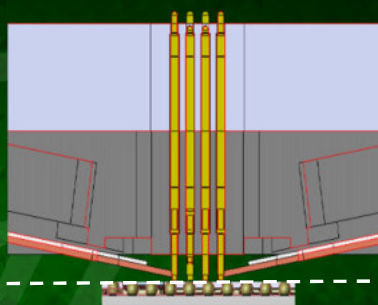
xWave Wafer Test
